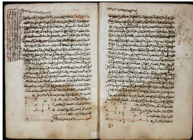
Figure 8: A page from a copy of ‘The Compendious Book on Calculation by Restoration and Balancing’ showing a geometric justification.
