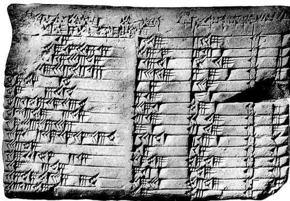
Figure 5: Plimpton 322 is a Babylonian clay tablet, notable as containing an example of Babylonian mathematics. It has number 322 in the G.A. Plimpton Collection at Columbia University.
