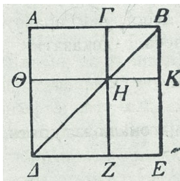
Figure 6: A diagram taken from a copy of Euclid's Elements Book II Proposition 4.
