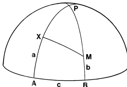
Figure 3: The problem of finding the direction of Mecca M from a point X requires find the angle which XM makes with PXA. ( D. King, The Sacred Direction in Islam. )
